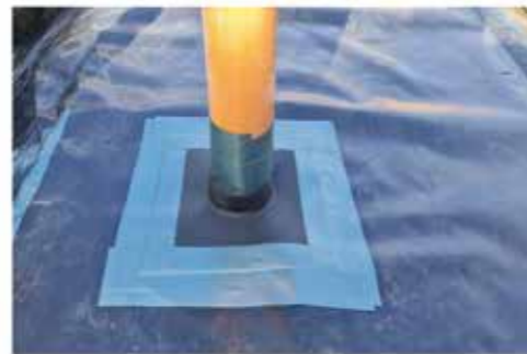
Tape flanges to membrane using HCR Foil Girth Tape.
