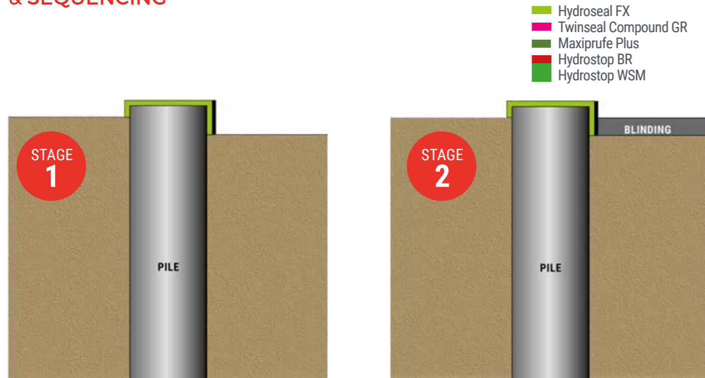
STAGE 1 Coat pileheads with Hydroseal FX and place Correx Board against the basement side of piles.
