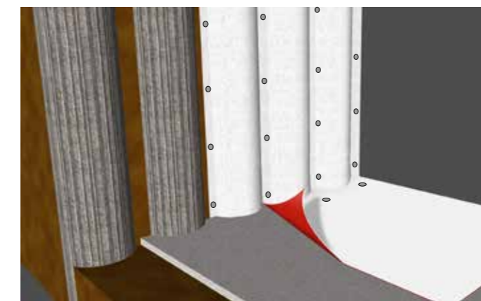
Trim horizontal membrane to blinding and fix tightly into the contours of the piles. Also fix wall membrane tightly into the contours of the piles with Metal Washer Fixings.
