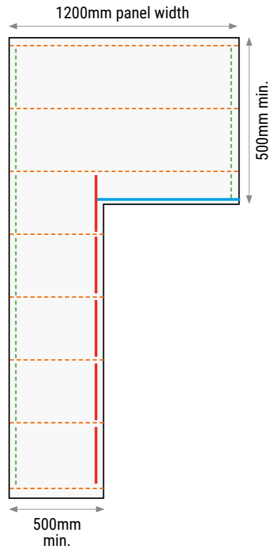
Tolerances for cutting VOID-TEK panels
