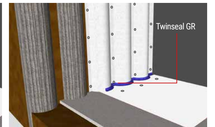
Apply 3mm thick x 100mm wide strip of Twinseal Compound GR along base of wall, sealing between slab and wall membrane.
