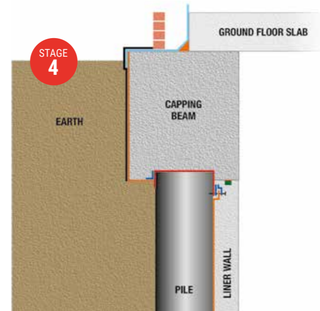
When capping beam is cast, and basement excavation is taking place, remove the Correx board exposing the Hydroprufe LG ready to connect the membrane.
