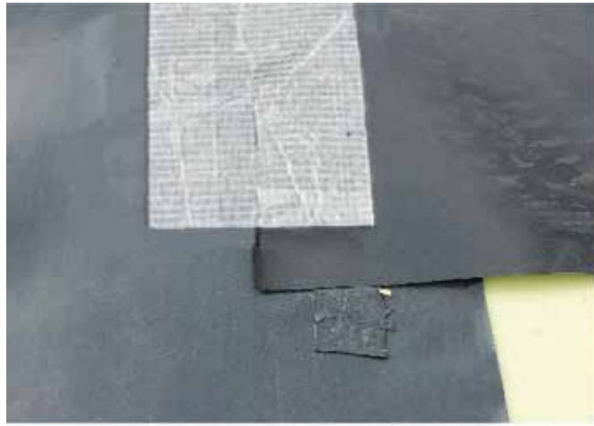
Minimum overlap should be 100mm. Laps to be sealed with 30mm HCR Butyl Tape within the lap and Girth Tape on the overlap. Laps should be rolled with a soft roller to ensure the tapes are fully bonded.
