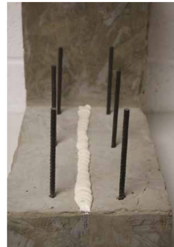
Apply 8mm bead of Hydrostop WSM to substrate.
