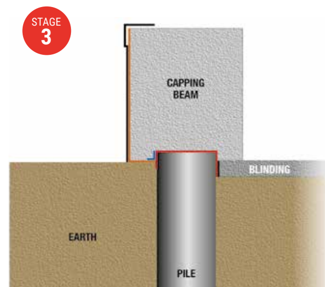
Install membrane to the outside of the pilehead and capping beam and seal the membrane to the pile head with Twinseal Compound GR. Install Protection Board 600 to outside of capping beam, prior to backfilling.
